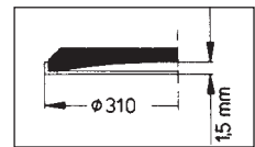
XMD 310.819
